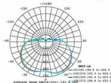
LUMINOUS INTENSITY DISTRIBUTION DIAGRAM 50W
