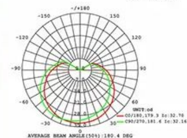
LUMINOUS INTENSITY DISTRIBUTION DIAGRAM 9W Green
