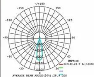
LUMINOUS INTENSITY DISTRIBUTION DIAGRAM 33W
