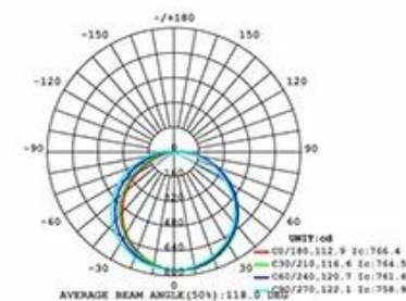
LUMINOUS INTENSITY DISTRIBUTION DIAGRAM Oval
