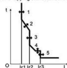
Electronic tripping characteristics curve
