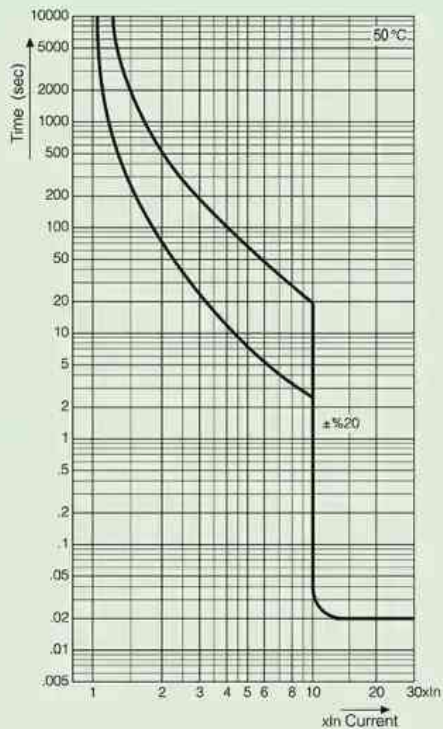
Thermal magnetic fixed type circuit breaker
