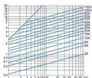
Prospective current I_p(kA) (symmetrical effective value) → Characteristic of cut-off current of "gG" fuse link
