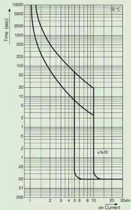
Thermal magnetic adjustable type circuit breaker
